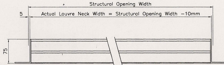
Sectional Plan On Arrow B.B.
