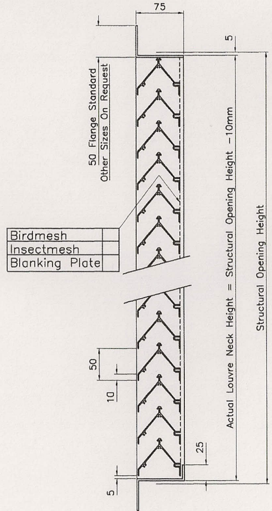
Sectional Elevation On Arrow A.A.
