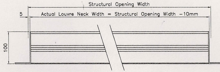
Sectional Plan On Arrow B.B.
