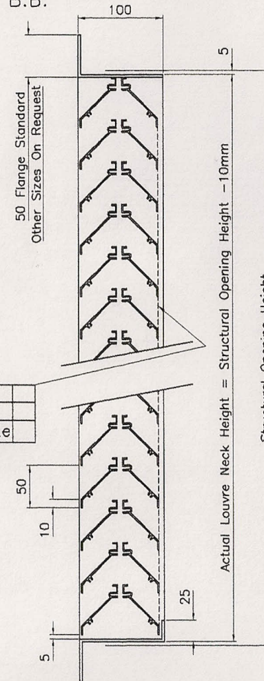
Sectional Elevation On Arrow A.A.
