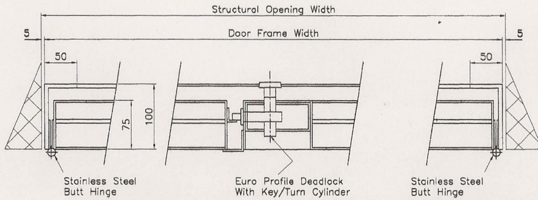
PLAN Section On B.B
