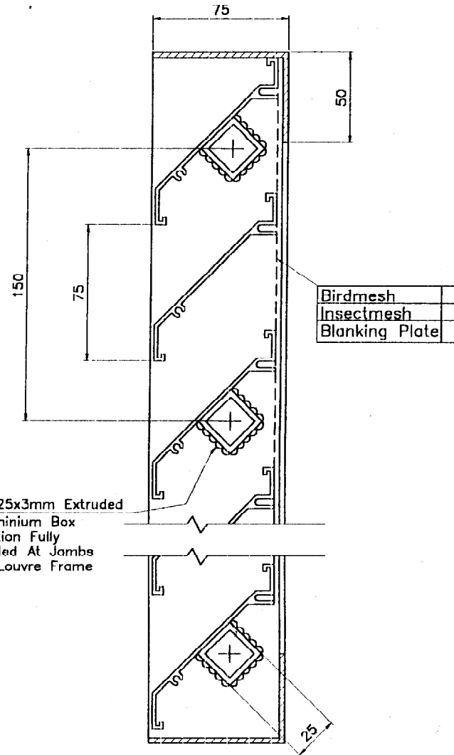
Sectional Side Elevation
