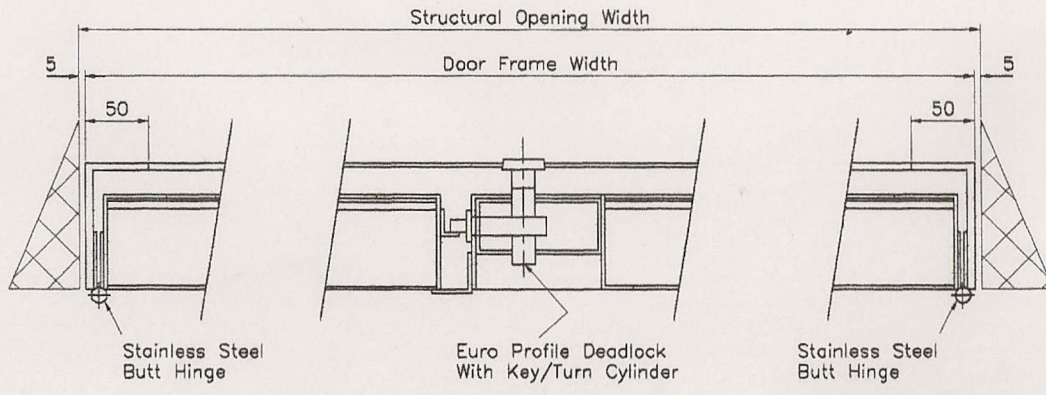
PLAN Section On B.B
