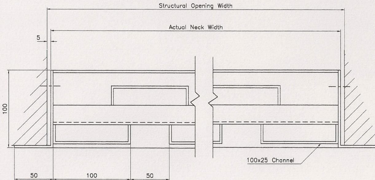
Sectional Plan At Jamb
