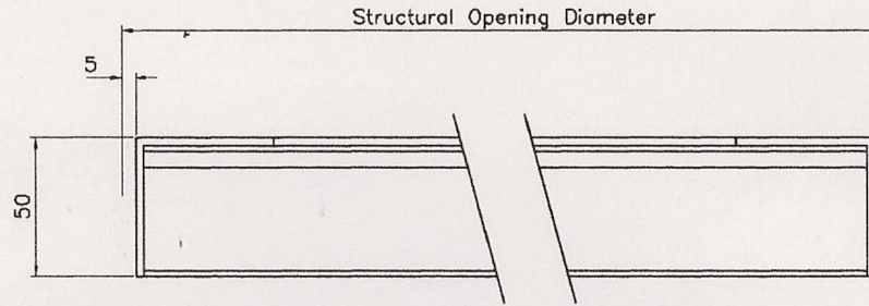
Sectional Plan On Arrow B.B.
